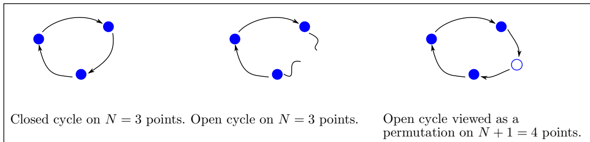
FIGURE 2. Open cycles as permutations on N + 1 points.
