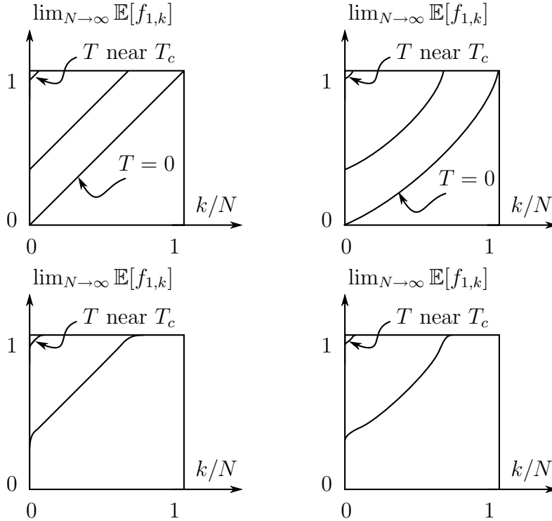
FIGURE 1. Qualitative behavior of \lim_{N \rightarrow \infty} \mathbb{E}[f_{1,k}] as a function of k/N in the non-interacting (upper left) and non-spatial large- \alpha Ewens-interacting (upper right) cases. Lower left and lower right show the behavior for finite N .
